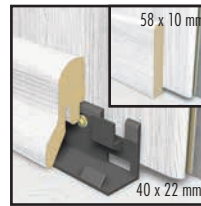
Skirting boards | Fußleisten 40 x 22 x 2600 mm (EX XXXX FUSS2240) 58 x 10 x 2600 mm (EX XXXX FUSS1058)
